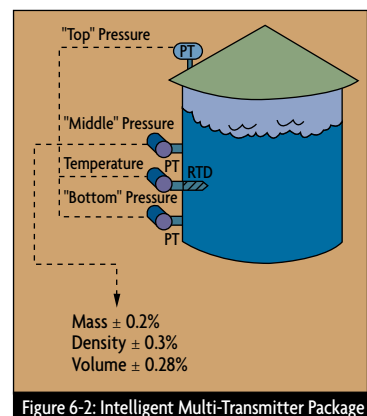
Figure 6-2: Intelligent Multi-Transmitter Package
