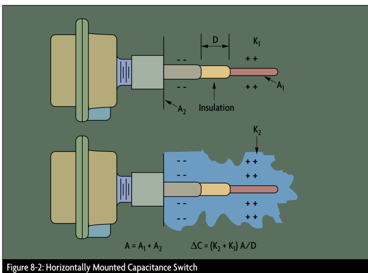
Figure 8-2: Horizontally Mounted Capacitance Switch
