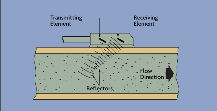
Figure 4-8: Clamp-On Ultrasonic Flowmeter
