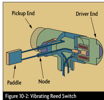
Figure 10-2: Vibrating Reed Switch
