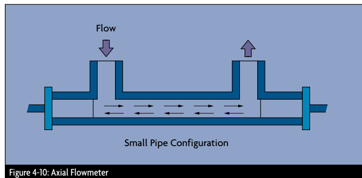
Figure 4-10: Axial Flowmeter
